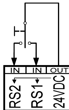
Fig.6 Remote start
